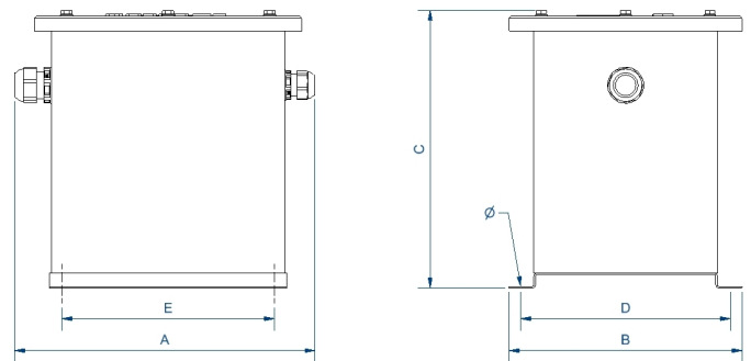
Dimensions (AxBxCxDxE): 240x235x260x212x218 mm 7φ
