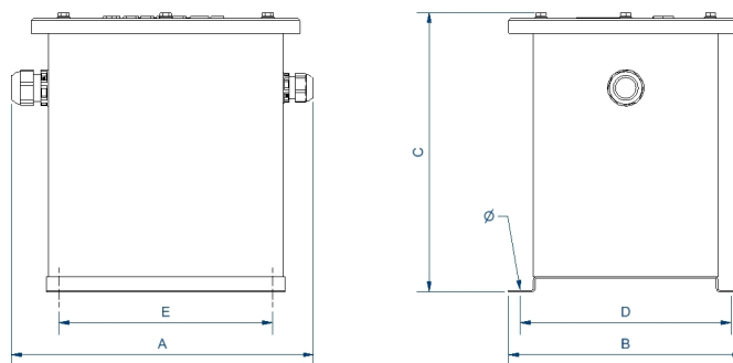
Dimensions (AxBxCxDxE): 260x272x310x250x238 mm 7Ø
