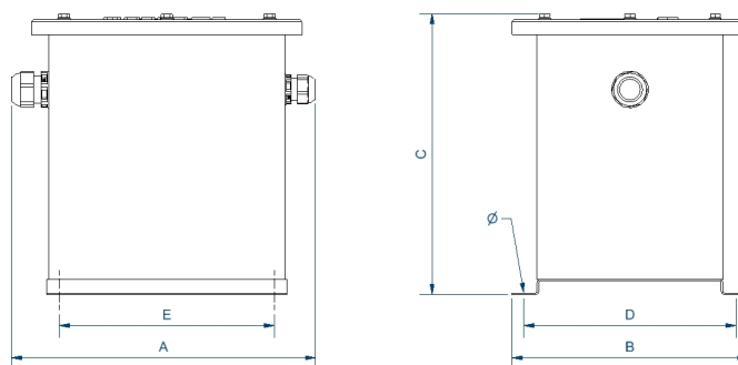
Dimensions (Ax BxCxDxE): 150x165x190x145x125 mm 7Ø
