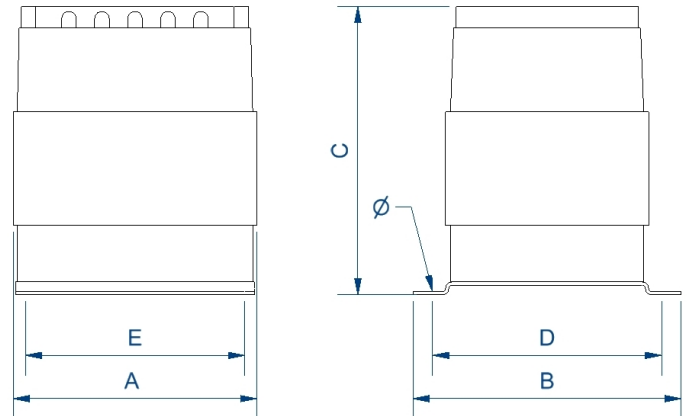
Dimensiones (AxBxCxDxE): 75x96x100x80x56 mm 6Ø
