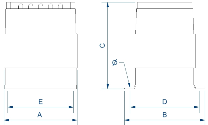
Dimensions (AxBxCxDxE): 75x97x84x80x56 mm 6Ø
