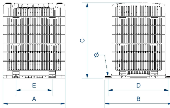
Dimensions (AxBxCxDxE): 214x225x284x195x175 mm \varnothing
