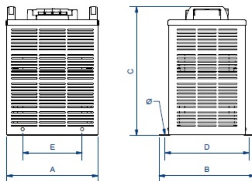
Dimensions (AxBxCxDxE): 252x260x349x233x223 mm 7Ø
