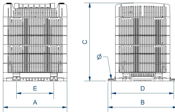
Dimensions (AxBxCxDxE): 252x260x349x233x223 mm 7Ø
