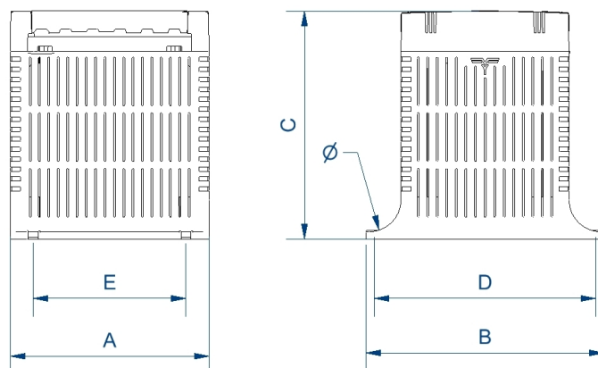
Dimensions (AxBxCxDxE): 136x162x180x146x104 mm 6Ø
