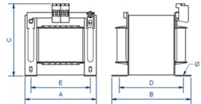
Dimensions (AxBxCxDxE): 150x135x135x102x125 mm 8
