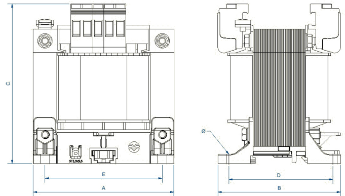
Dimensions (AxBxCxDxE): 108x98x109x83x90 mm 6
