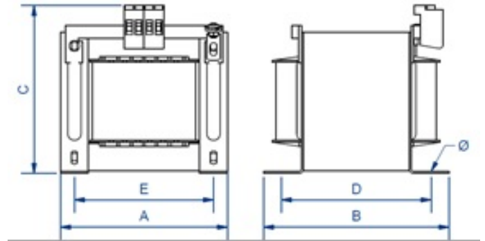
Dimensions (AxBxCxDxE): 126x110x115x75x106 mm 8
