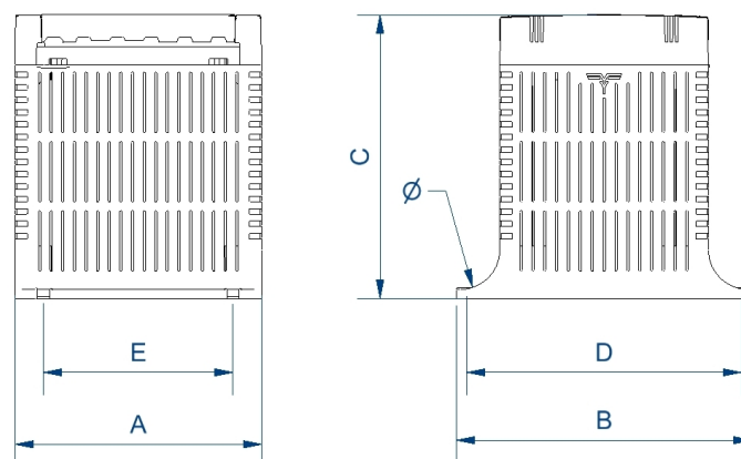
Dimensions (AxBxCxDxE): 84x101x98x89x55 mm 5 \varnothing
