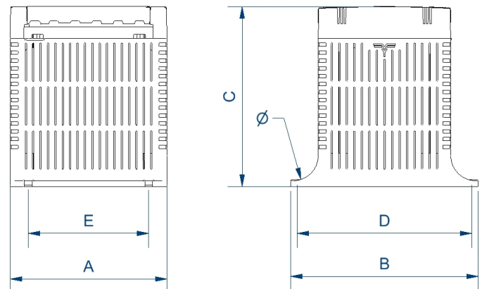
Dimensions (AxBxCxDxE): 106x123x122x111x74 mm 5∅
