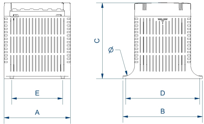
Dimensions (AxBxCxDxE): 84x101x98x89x55 mm 5Ø
