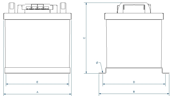
Dimensions (AxBxCxDxE): 233x241x244x219x175 mm 7Ø
