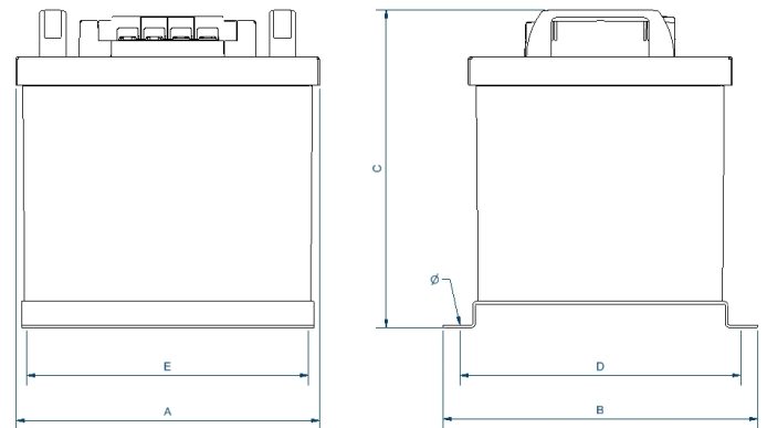
Dimensions (AxBxCxDxE): 233x241x274x219x175 mm 7Ø
