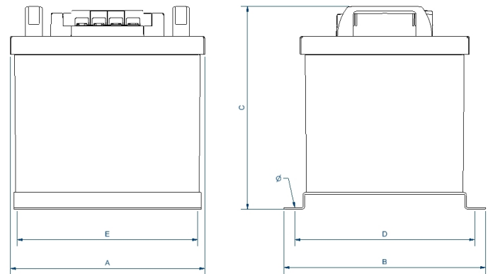
Dimensions (AxBxCxDxE): 233x241x314x219x175 mm 7Ø
