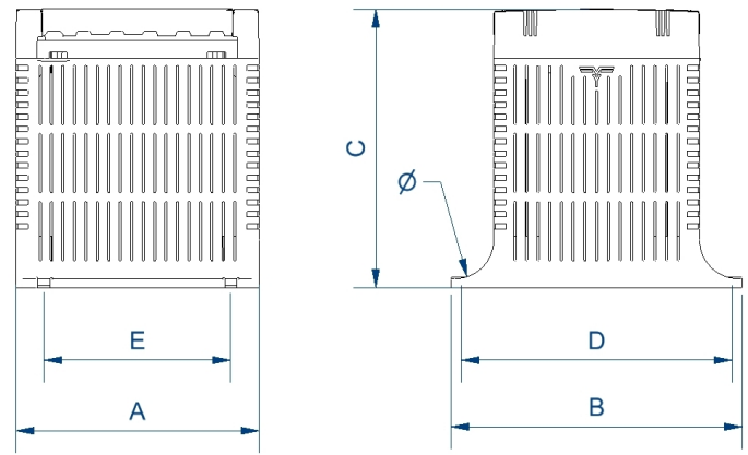
Dimensions (AxBxCxDxE): 118x138x132x122x88 mm 5∅
