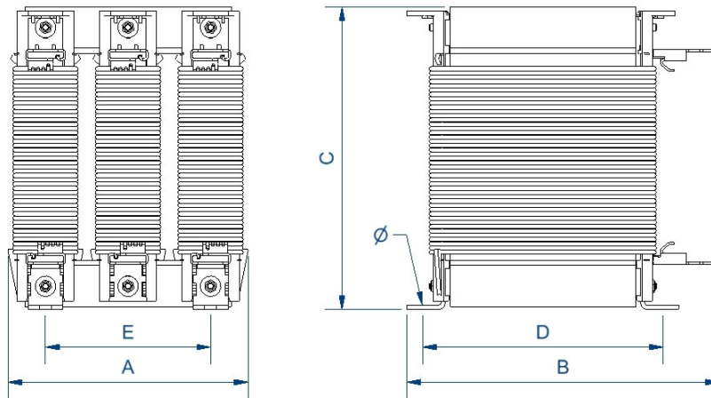
Dimensions (AxBxCxDxE): 180x160x220x105x120 mm 9Ø
