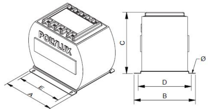
Dimensions (AxBxCxDxE): 210x198x185x178x173 mm 7Ø
