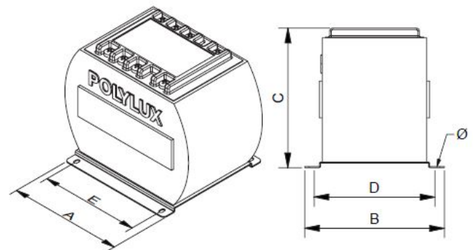
Dimensions (AxBxCxDxE): 135x145x108x125x102 mm 7 
