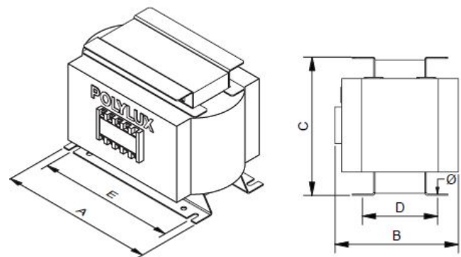
Dimensions (AxBxCxDxE): 280x190x205x100x250 mm 9̊
