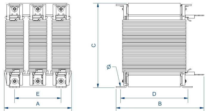
Dimensions (AxBxCxDxE): 180x205x220,25x144x120 mm 6Ø
