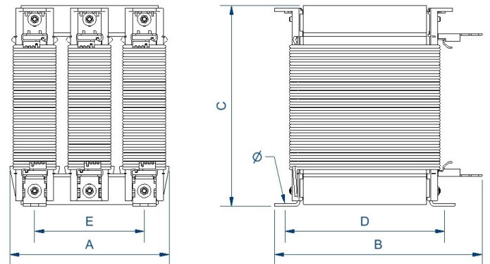
Dimensions (AxBxCxDxE): 180x150x220,25x89x120 mm 6Ø
