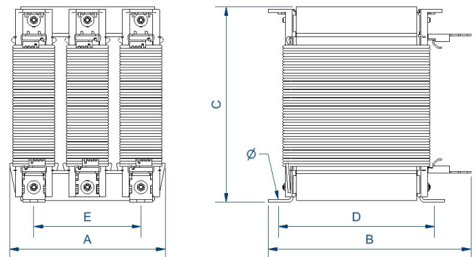
Dimensions (AxBxCxDxE): 180x165x220,25x104x120 mm 6Ø
