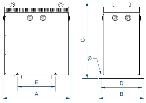
Dimensiones (AxBxCxDxE): 528x418x644x375x345 mm 12Ø
