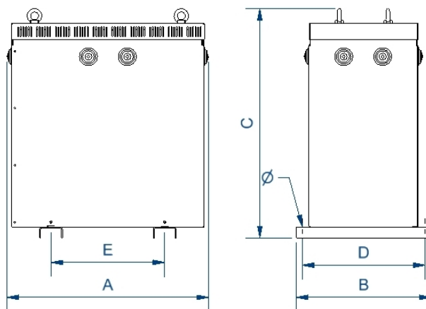
Dimensiones (AxBxCxDxE): 528x418x644x375x345 mm 12Ø
