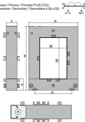
Dimensions (AxBxCxDxE): 144x50x185 mm
