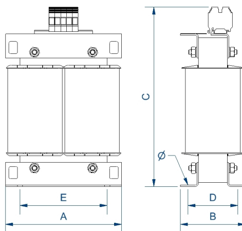
Dimensions (AxBxCxDxE): 320x194x460x126x240 mm 11Ø
