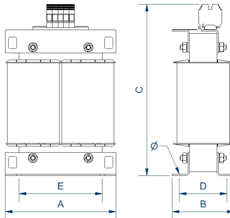
Dimensions (AxBxCxDxE): 320x214x465x146x240 mm 11Ø
