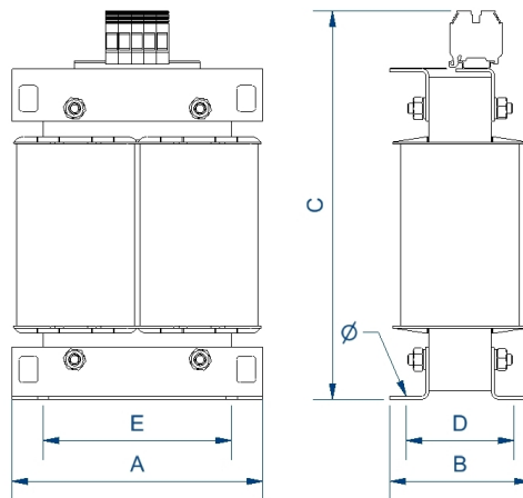
Dimensions (AxBxCxDxE): 200x164x320x128x154 mm 9Ø
