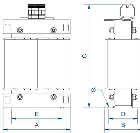
Dimensions (AxBxCxDxE): 240x144x355x108x180 mm 11Ø
