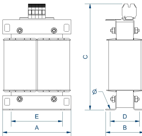
Dimensions (AxBxCxDxE): 240x164x372x128x180 mm 11Ø
