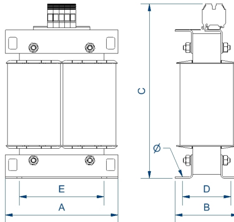
Dimensions (AxBxCxDxE): 280x175x421x126x210 mm 11Ø
