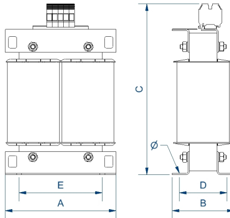
Dimensions (AxBxCxDxE): 280x195x421x146x210 mm 11Ø
