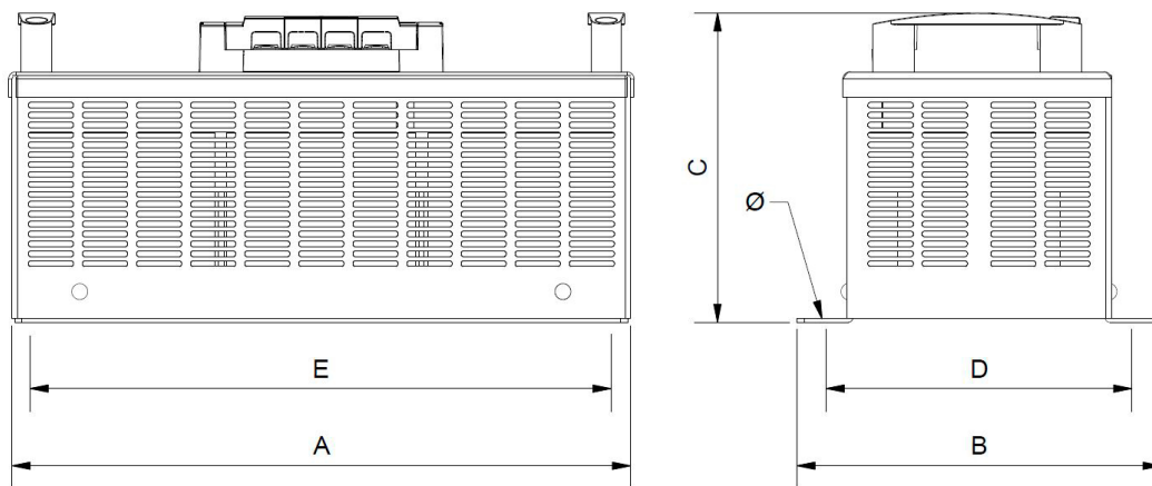
Dimensions (AxBxCxDxE): 350x200x220x170x325 mm 6φ
