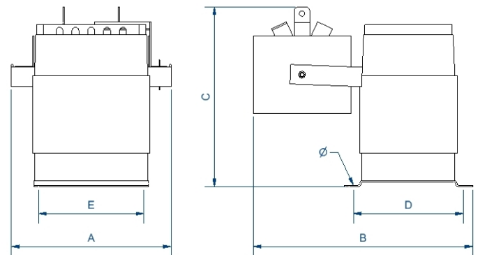
Dimensions (AxBxCxDxE): 191x165x250 mm 7Ø
