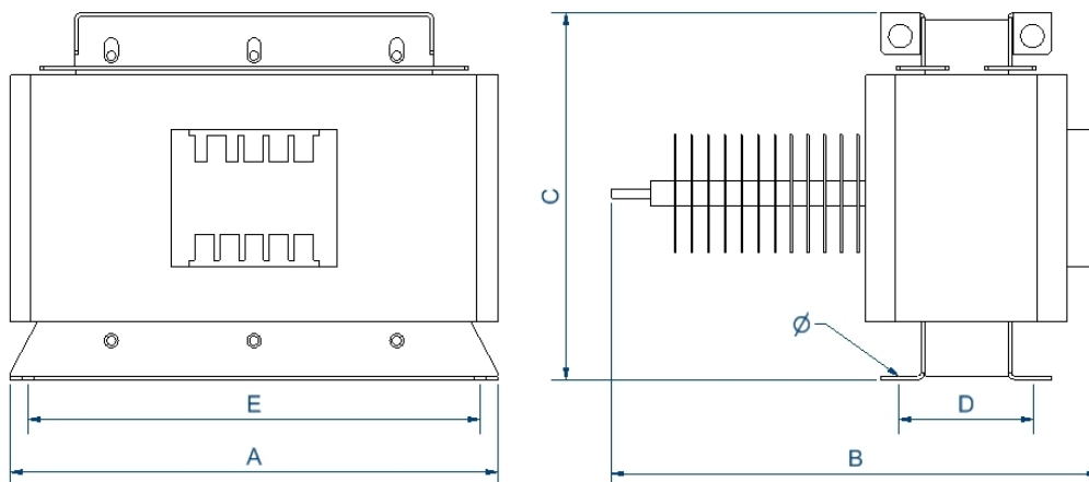
Dimensions (AxBxCxDxE): 340x440x255x96x310 mm 9 
