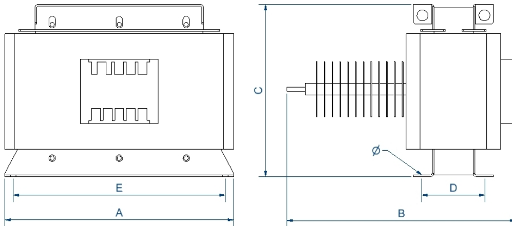
Dimensions (AxBxCxDxE): 340x470x255x126x310 mm 9 
