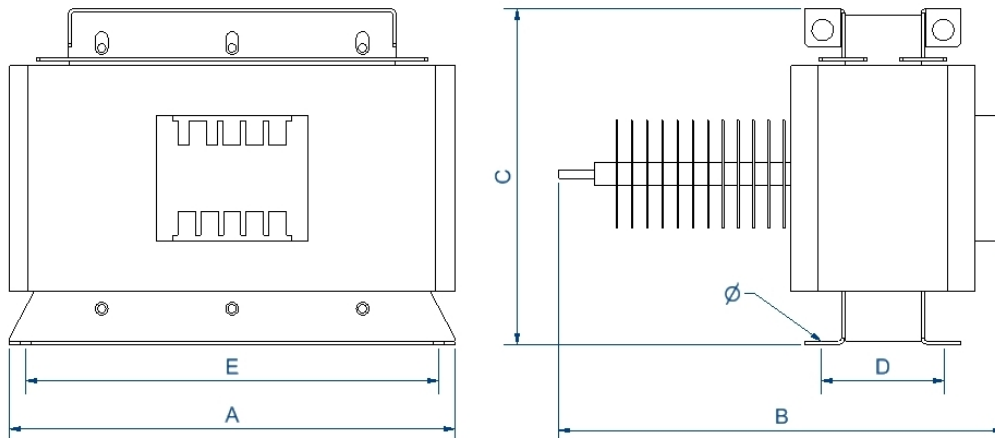
Dimensions (AxBxCxDxE): 410x460x305x116x380 mm 11 
