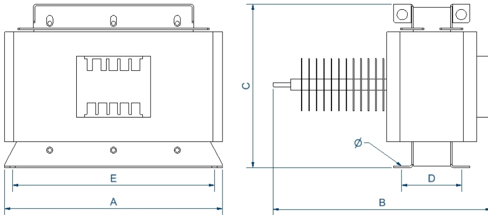
Dimensions (AxBxCxDxE): 490x780x355x142x460 mm 11 
