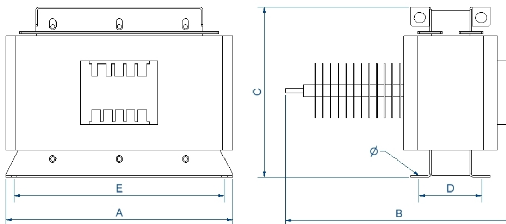
Dimensions (AxBxCxDxE): 490x780x355x142x460 mm 11Ø
