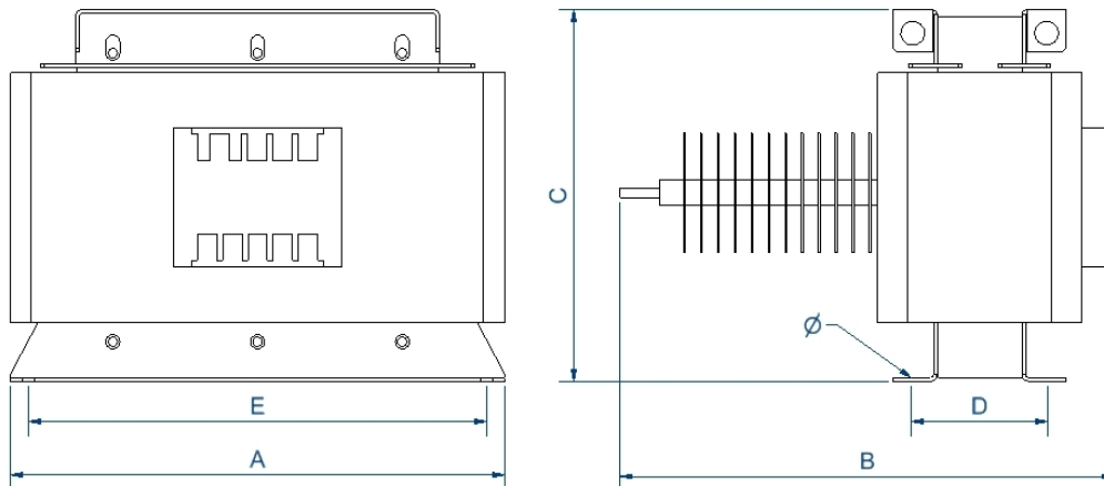
Dimensions (AxBxCxDxE): 490x820x355x162x460 mm 11 
