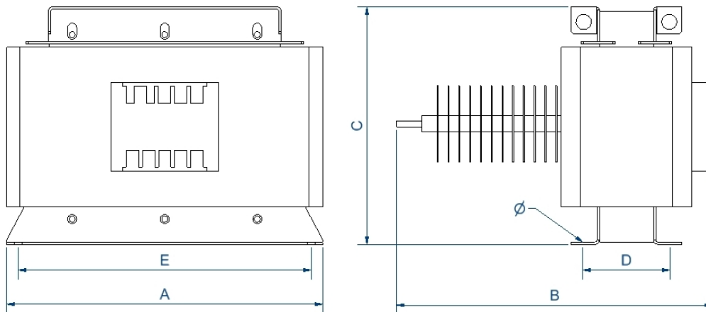
Dimensions (AxBxCxDxE): 280x365x220x80x250 mm 90°
