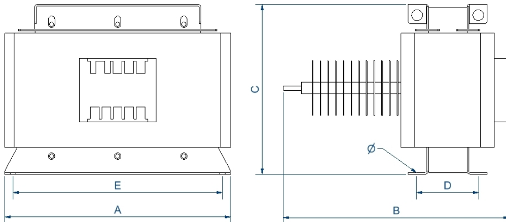
Dimensions (AxBxCxDxE): 540x1070x405x144x510 mm 11 
