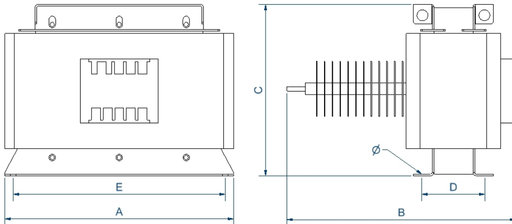
Dimensions (AxBxCxDxE): 490x780x355x142x460 mm 11∅
