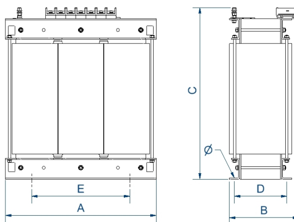
Dimensiones (AxBxCxDxE): 670x360x690x250x426 mm 13Ø
