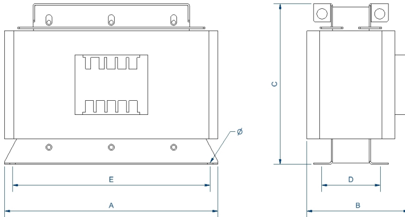
Dimensions (AxBxCxDxE): 280x158x205x100x250 mm 9Ø
