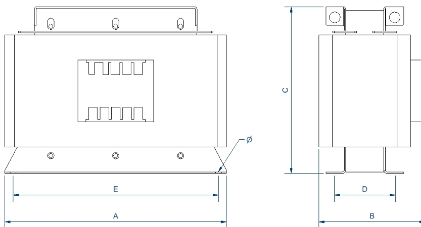
Dimensions (AxBxCxDxE): 280x158x205x100x250 mm 9Ø
